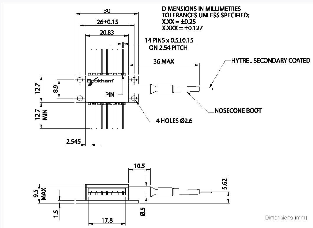
Figure 1: Outline Drawing
