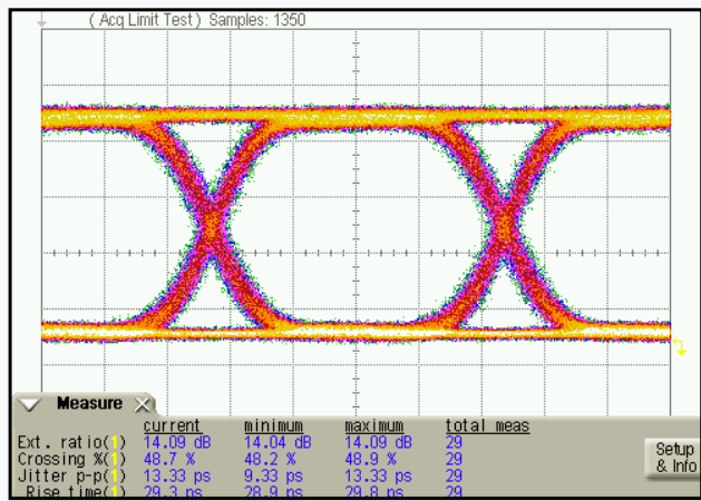
Eye Diagram
